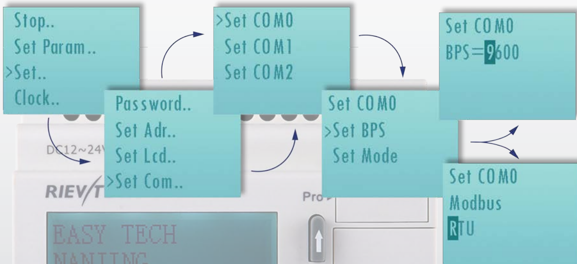
Universal Port - Serial COM0 Can work as RS232/USB
