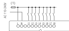
[Digital Input - Power AC]
